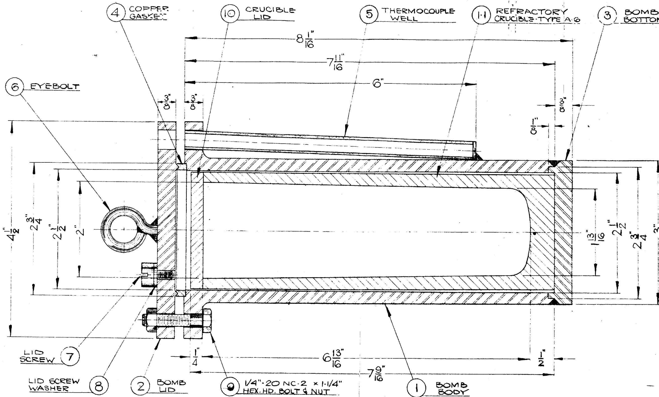
FIGURE 7(a) 250 GRAM BOMB ASSEMBLY SCALE : FULL SIZE
